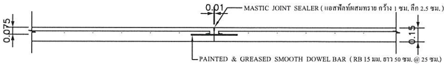
CONTRACTION JOINT
